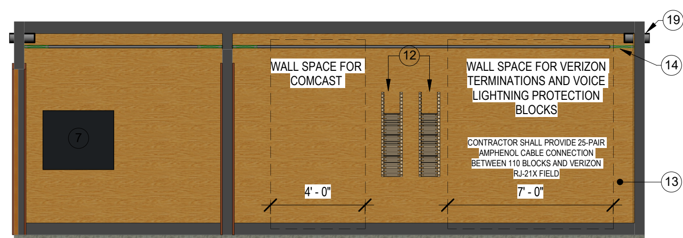
③ MDF & E-MDF - EAST WALL ELEVATION 1/4" = 1'-0"
