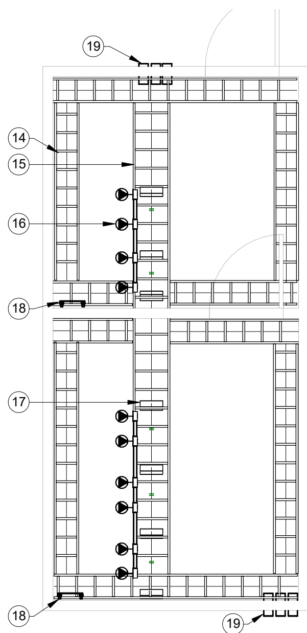
② IDF & E-IDF REFLECTED CEILING PLAN 1/4" = 1'-0"
