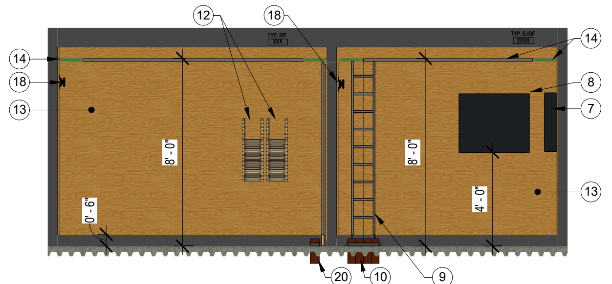
③ IDF, E-IDF - WEST WALL ELEVATION 1/4" = 1'-0"
