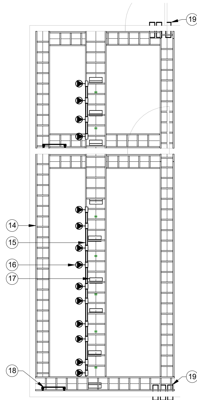
② MDF & E-MDF RCP 1/4" = 1'-0"
